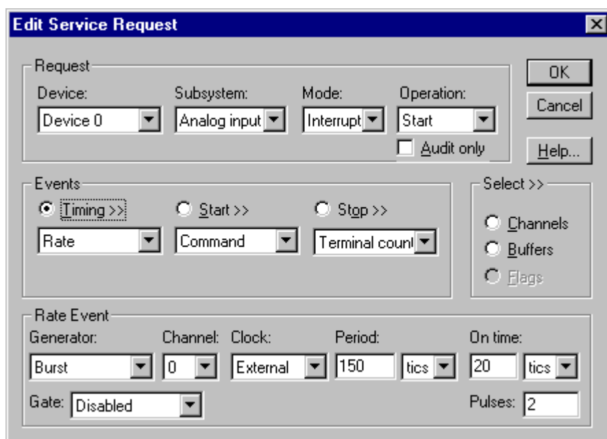
How to set up the DAS-1800 Series for burst mode sampling using an external clock.
