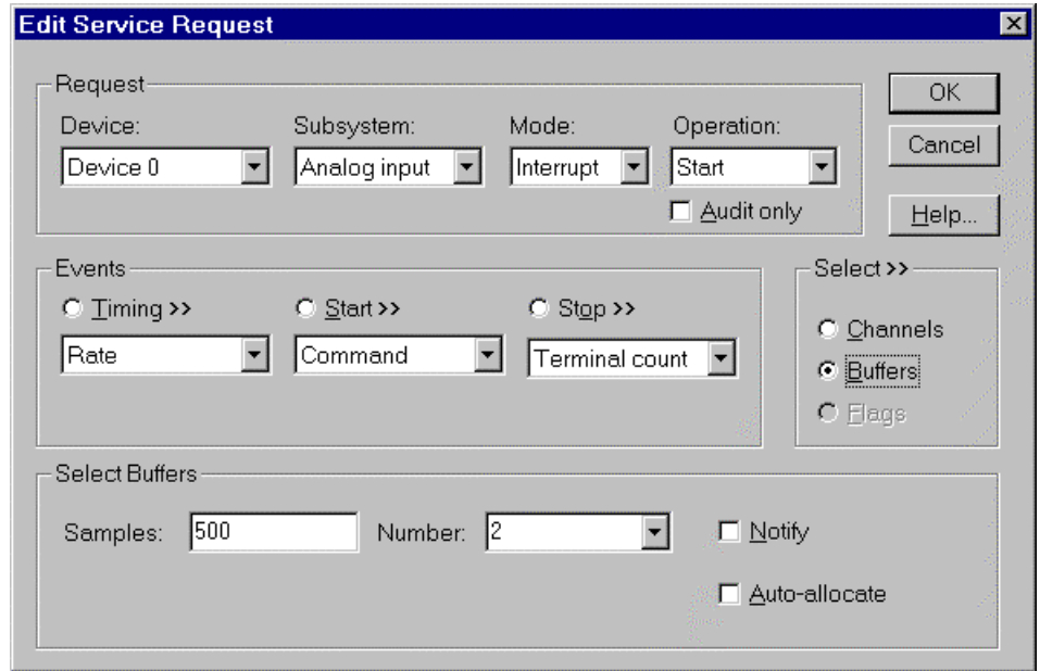
How to set up the DAS-1800 Series to store samples in buffers.
