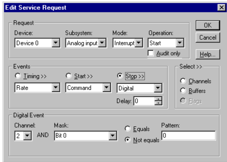
How to set up the DAS-1800 Series for pre-triggered analog input.
